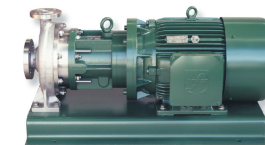
DICKOW MAGNETIC DRIVEN PUMPS Magnetic Drive metallic pumps including high temperature, ANSI, DIN, API-685 centrifugal, side channel and multi-stage used for hot oils, liquefied gases and volatile and corrosive liquids.
