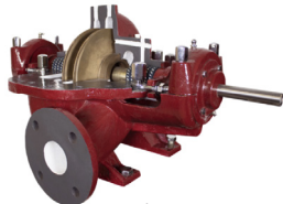
380 series HH Two-stage horizontal split case pumps
