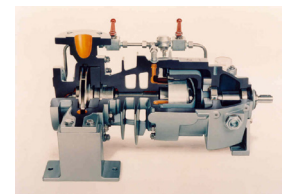
DICKOW MAGNETIC DRIVEN PUMPS Magnetic Drive metallic pumps including high temperature, ANSI, DIN, API-685 centrifugal, side channel and multi-stage used for hot oils, liquefied gases and volatile and corrosive liquids.
