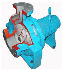
DEAN PUMPS Inline, ANSI, high temperature, vertical sump, self-priming, API610 (5th edition) Magnetic drive ANSI and hot oil pumps.
