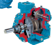
SEALLESS: Magnetically driven rotary sliding vane.
